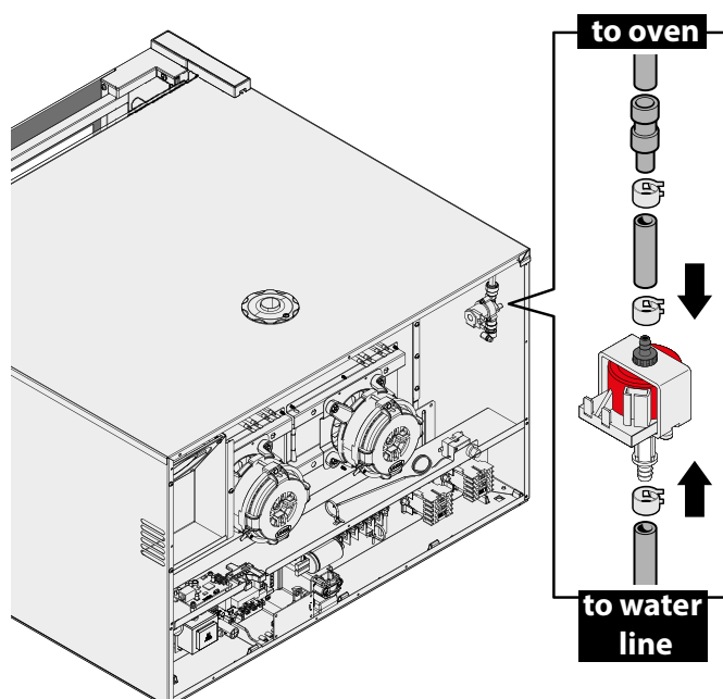
Fig. 5 Steam pump
