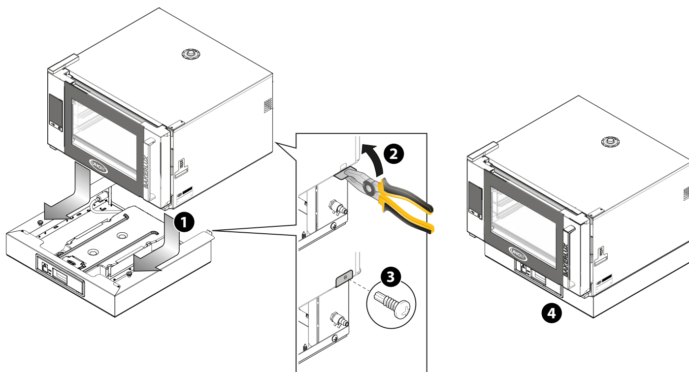
Fig. 6 Water tank
