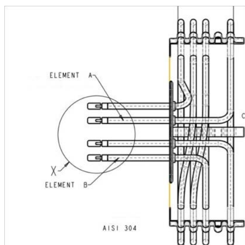
Fig. 10 Heating element
