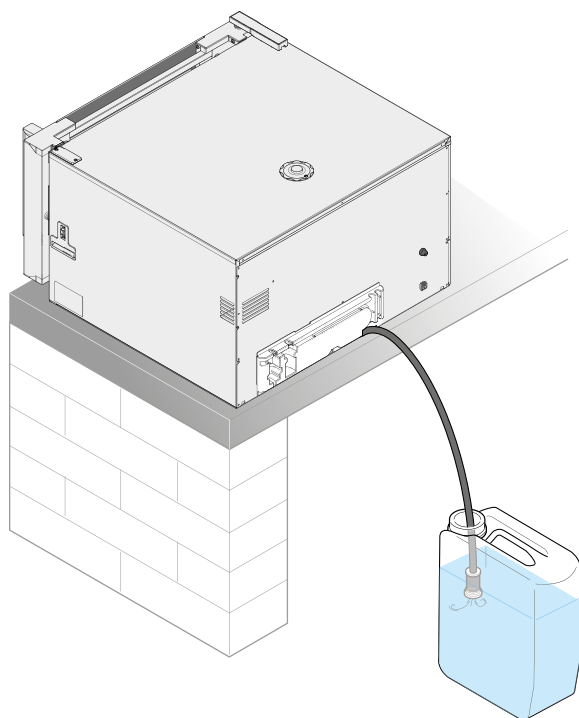
Fig. 6 Water tank
