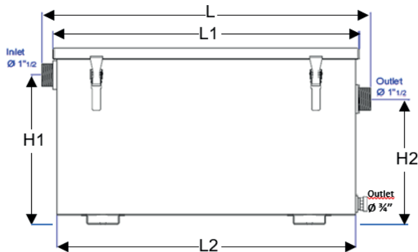
VISTA FRONTAL
